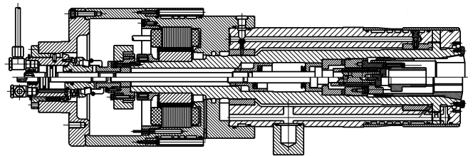
Shown with integral drawbar, cooling jacket, collet mechanism and encoder
